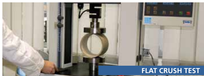
RADIAL TEST
